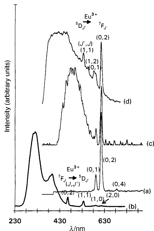
Fig. 5 Luminescence and excitation spectra of Eu( H2 ) 3 (NO 3 ) 3 ·2H 2 O ( 4 ): (a) emission spectrum (300 K); λ exc = 300 nm, gating time t g = 1 ms, delay time t d = 1 ms; (b) excitation spectrum (300 K); λ em = 610 nm, [Eu 3+ ( 5 D 0 )] = 1 ms, t d = 1 ms; (c) emission spectrum (77 K); λ exc = 300 nm, t g = 1 ms, t d = 12 ms; (d) emission spectrum (77 K); λ exc = 300 nm, t g = 0.01 ms, t d = 0.02 ms
