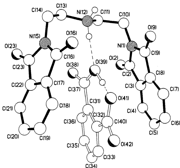
Fig. 3 Horseshoe conformation of DPDAH + and the trapped hydrogen phthalate anion in DPDAH-HP·1.75H 2 O
