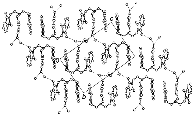
Fig. 4 Extended H-bonding in DPDAH-HP·1.75H 2 O leading to a layer motif
