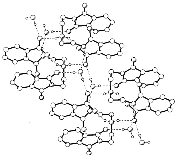
Fig. 2 Centrosymmetrically related hydrogen bonded 'dimer pairs' of \text{H}_2\cdot\text{H}_2\text{O} N(amine) \cdots O(carboxylate) 2.71 Å, H \cdots O 1.87 Å, N-H \cdots O angle 154°; N(amido) \cdots O(water) 2.83 Å, H \cdots O 1.99 Å; N-H \cdots O angle 156°; O(water) \cdots O(phthalimido) 2.84 Å, H \cdots O 1.98 Å, O-H \cdots O angle 159°
